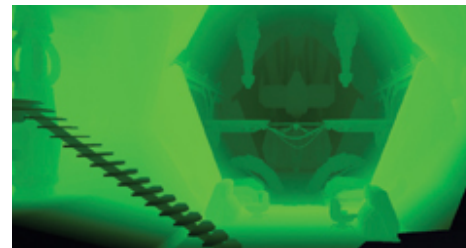
Depth
