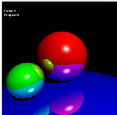
Ray Tracing
