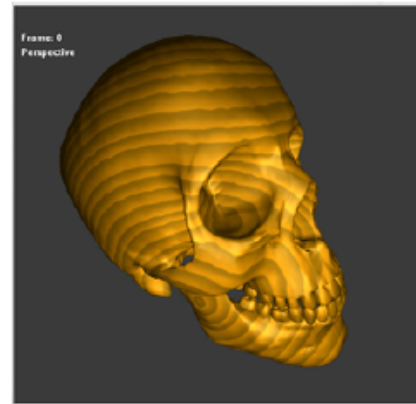
Solid Textures
