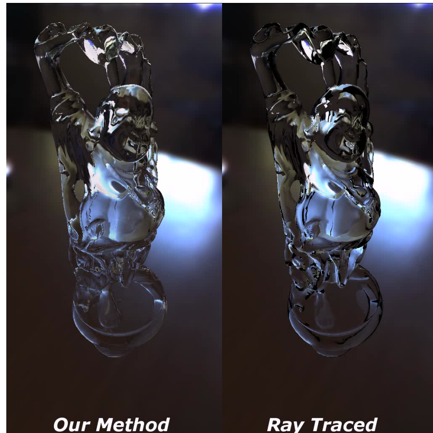
Lichtbrechung (1 bounce)
